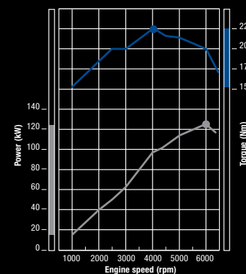
2.4L MIVEC DOHC Engine
